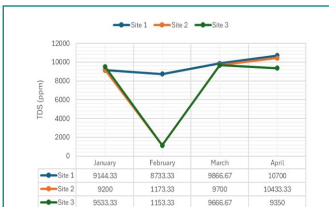
Figure 5: The TDS of water in Navotas river during the four-month sampling period.
